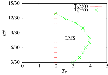
FIG. 10. (Color online) t/N-T_S diagram of the domain where the local Mattis states are found at N=30 and a fixed T_J=0.5 \times 10^{-3} . The points on the boundary of the domain are estimated by the values of T_S at which \Phi_2 drops from 1, as in Fig. 9(c), and the line is guide to eyes.
