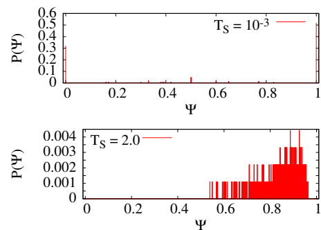
FIG. 13. (Color online) The fitness distribution of mutated \mathbf{J} with mutation rate \mu=0.1 , which are generated from the evolved genotypes at T_S=10^{-3} and at T_S=2.0 at N=15 . The distribution is obtained by 100 types of mutated \mathbf{J} .
