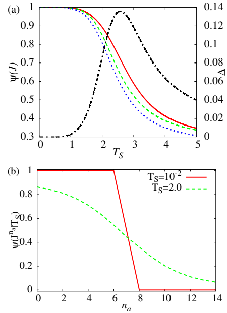
FIG. 11. (Color online) (a) The T_S dependence of the fitness of the Mattis state (bold line, \Phi_1 = \Phi_2 = \Phi_3 = 1 ), one of the local Mattis states (dashed line, \Phi_1 = \Phi_2 = 1, \Phi_3 = 0.89 ), and one of the target-frustrated states (dotted line, \Phi_1 = 0.333, \Phi_2 = 1, \Phi_3 = 0.89 ), plotted on the left axis. The dashed-dotted line represents the difference \Delta between the fitness of the Mattis state and that of the target-frustrated state; \Delta is plotted on the right. (b) The fitness of \tilde{\mathbf{J}}^{n_a} adapted at T_S=10^{-2} (solid line) and T_S=2.0 (dashed line) with N=15 and t=3 , plotted as a function of the number n_a of flipped bonds of \tilde{\mathbf{J}}^{n_a} . At low T_S , the fitness decreases rapidly for n_a=7 and decreases gradually at intermediate T_S .
