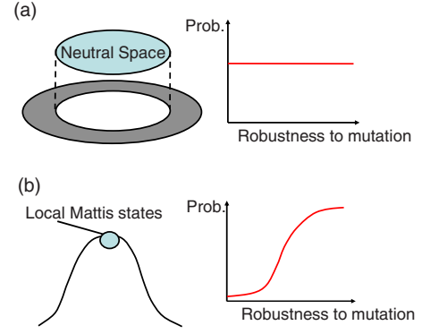
FIG. 12. (Color online) Schematic representation of the fitness landscape and the probability distribution of the robustness to mutation estimated from the fitness landscape. (a) At low T_S , the genotypes that satisfy the condition W_{\Psi}(E_0(\mathbf{J}))=W(E_0(\mathbf{J})) exist in the neutral space, where the fitness attains its highest value. The local Mattis states also exist in the neutral space, but they constitute a negligible fraction compared to the frustrated genotypes. The neutral space is surrounded by nonadapted genotypes with sharp boundaries, as in Fig. 11(b). The genotypes around the edge of the neutral space that have very low robustness to mutation survive in an evolutionary sense, similar to the robust genotypes located at the center of neutral space, that are much fewer in number. (b) For T_S with T_S^1 \leq T_S \leq T_S^2 , the degeneracy observed at low values of T_S is split, and the local Mattis states have the highest fitness. The fitness of the local Mattis state decreases continuously with increasing mutation. There is a correlation between fitness and robustness, i.e., the local Mattis state with the highest fitness is the most robust to mutation, and the robust genotypes are selected preferentially.
