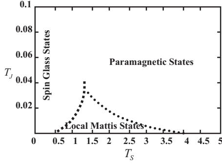
FIG. 6. Phase diagram of the evolved J_s at N=15 and t=3 . Three types of evolved J are defined on the basis of the value of the fitness and \Phi_2 . Their properties are summarized below in Table I.
