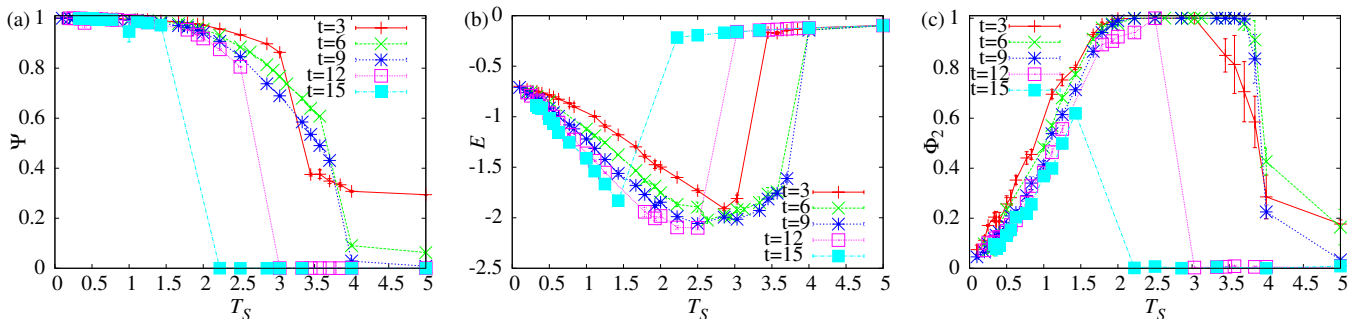
FIG. 9. (Color online) The T_S dependence of (a) the fitness, (b) the energy, and (c) \Phi_2 at N=30 and t=3, 6, 9, 12 , and 15. The temperature T_J is fixed at 0.5 \times 10^{-3} . The convergence value of the fitness (a) at T_S \rightarrow \infty is 2^{-t+1} .
