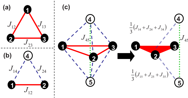
FIG. 3. (Color online) Definition of frustration in terms of the parameters \Phi_1 , \Phi_2 , and \Phi_3 for the case with three target spins ( t=3 ); S_i(i=1,2,3) are target spins and the remaining spins are nontargets. The bold lines depict the interactions between target spins ( \in J_{tt} ), the dashed lines depict those between target and nontarget spins ( \in J_{to} ), and the dotted lines depict those between nontarget spins ( \in J_{oo} ); (a) a triangle consists of three J_{tt} interactions; (b) a triangle consists of one J_{tt} interaction and two J_{to} interactions which are connected to the same nontarget spin; (c) a hexahedron that consists of all types of interactions. By summing up the target spins, it is represented as a triangle with a renormalized interaction.
