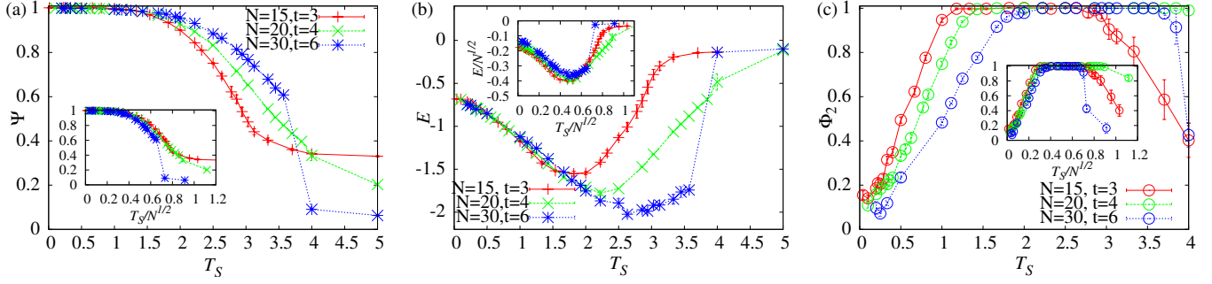
FIG. 8. (Color online) The T_S dependence of (a) the fitness, (b) the energy, and (c) the frustration parameter \Phi_2 at N=15 , t=3 , N=20 , t=4 and N=30 , t=6 . The temperature T_J is fixed at 0.5 \times 10^{-3} . The inset of each figure shows the dependence of each quantity on the temperature rescaled by \sqrt{N} . The vertical axis of the inset of (b) is also rescaled by \sqrt{N} .
