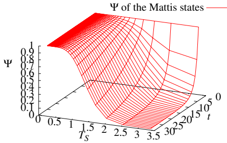
FIG. 14. (Color online) T_S and t dependence of the fitness \Psi(T_S, t) of the Mattis state at N=30 .
