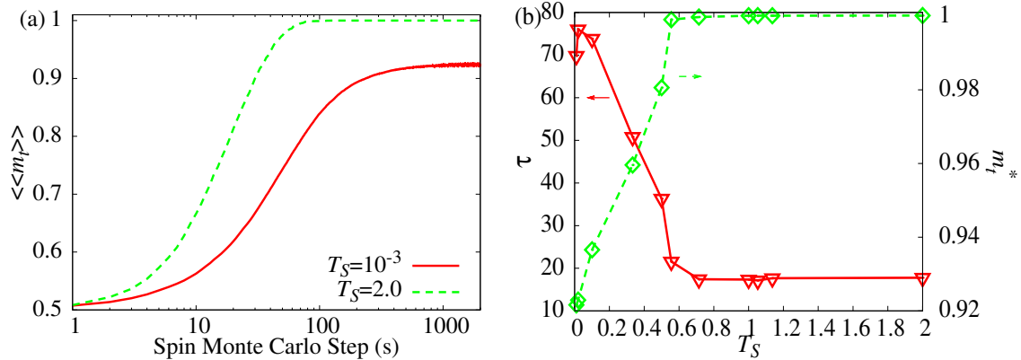
FIG. 7. (Color online) (a) Relaxation dynamics of the averaged magnetization of target spins, \langle\langle m_i \rangle\rangle , averaged over the adapted interactions J for T_S=10^{-3} (solid curve) and T_S=2.0 (dashed curve). The magnetization \langle\langle m_i \rangle\rangle is evaluated by calculating the average over 30 initial conditions for each J and 1000 different samples of J that are drawn from P(J, T_S, T_J=10^{-3}) . (b) The T_S dependence of the estimated convergent value of \langle\langle m_i \rangle\rangle , m_i^* on the right axis and the relaxation time \tau on the left. The relaxation time is estimated from the time constant of an exponential decay of \langle\langle m_i \rangle\rangle .
