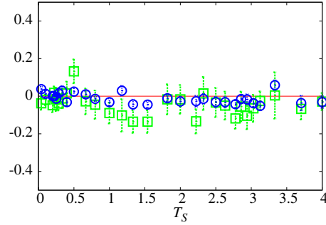
FIG. 5. (Color online) T_S dependence of the averages \overline{J_{to}} ( \square ) and \overline{J_{oo}} ( \circ ) for a fixed T_J=0.5 \times 10^{-3} .
